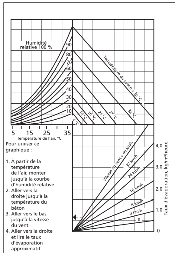
Figure 2.1.5, ACI 305, Hot Weather Concreting
