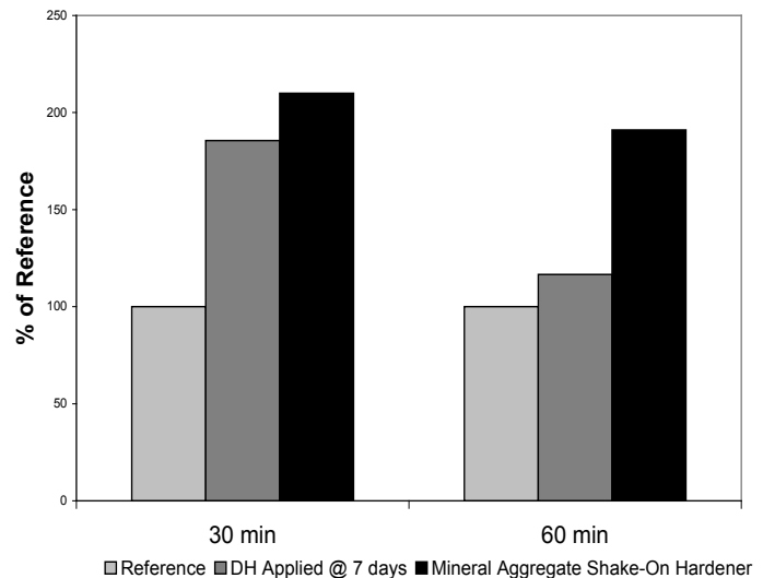
EUCO DIAMOND HARD ASTM C 779 Wear Resistance Results @ 28 Days
